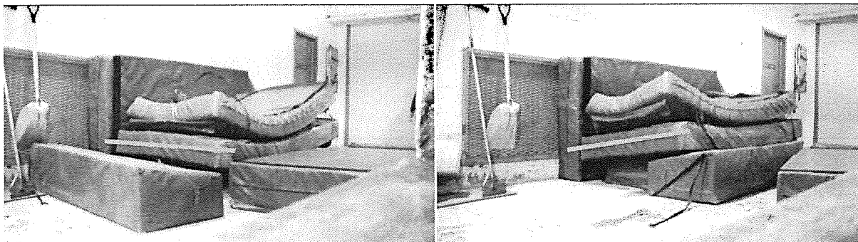
FIGURE 13 IMPACT WITH SHORT AND FULL MATS BEHIND
