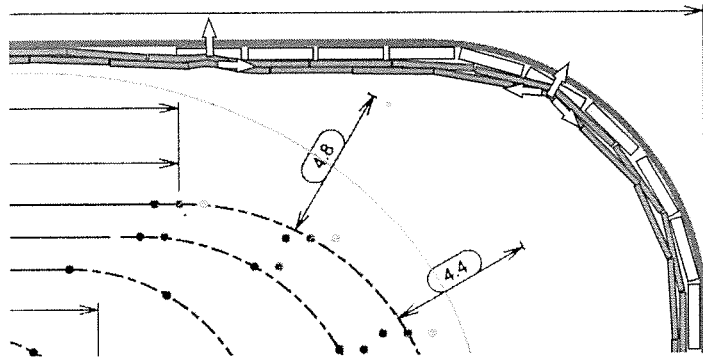
FIGURE 48. SIDE EFFECT ON THE TURN
