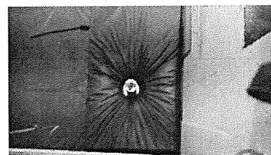
FIGURE 36 IMPACT CLOSE TO THE ICE AND IN THE MIDDLE OF THE MATS
