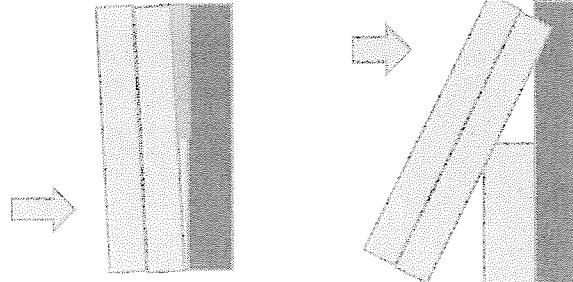
FIGURE 16 ROTATION OF THE TOP WITHOUT UPPER MATS
