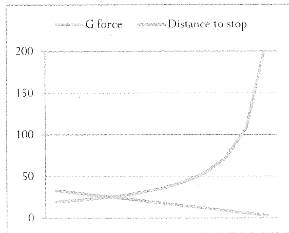
GRAPH 1 G FORCE FUNCTION OF THE DISTANCE TO STOP DURING CONTINUOUS DECELERATION
