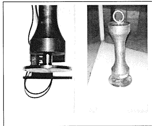
FIGURE 18 SNAPSHOCK ACCELEROMETER
