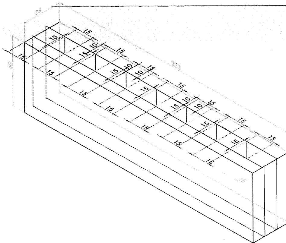
FIGURE 28 SHORT MAT QC
