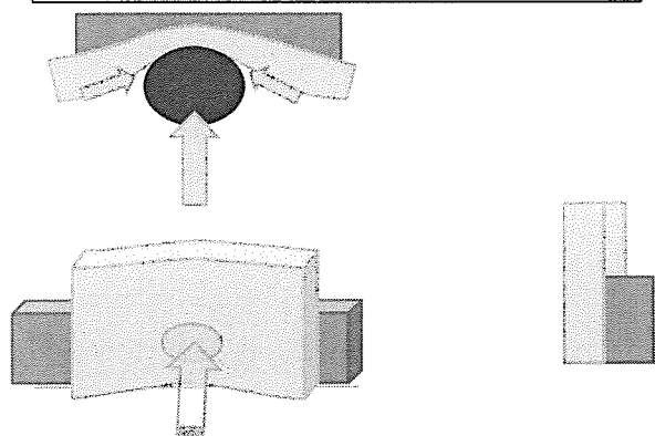
FIGURE 11 DEFORMATIONS WITH SHORT MAT BEHIND
